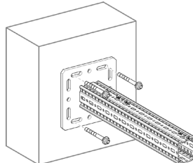
Part List 1 x Beam Bracket TKO F 80 4 x Anchors
